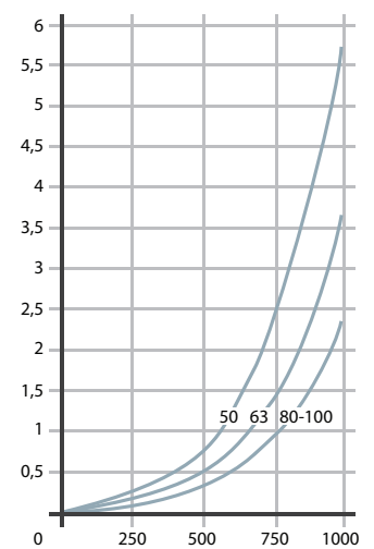
Deflection with 100 N load
