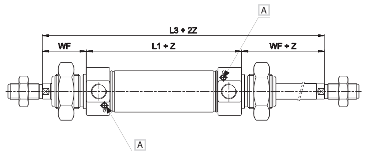
M151 D.A. Through piston rod with adjustable cushionings
