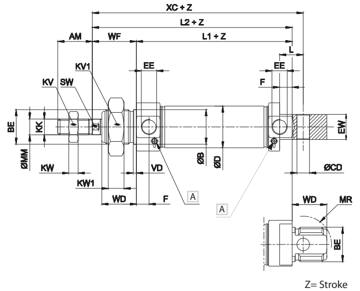
M150 D.A. With adjustable cushionings
